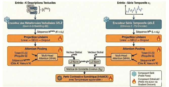
(b) Architecture globale.
